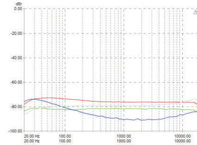
Figure 6.6 CMSweep @ 20 Hz -> 20 kHz (Measurement of a typical performance)
