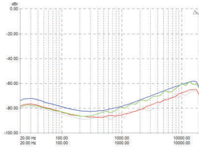
Figure 6.4 C-sweep @ 20 Hz -> 20 kHz (Measurement of a typical performance)
