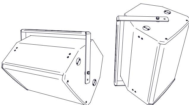
Mounting bracket for versions with option 'Installation'
