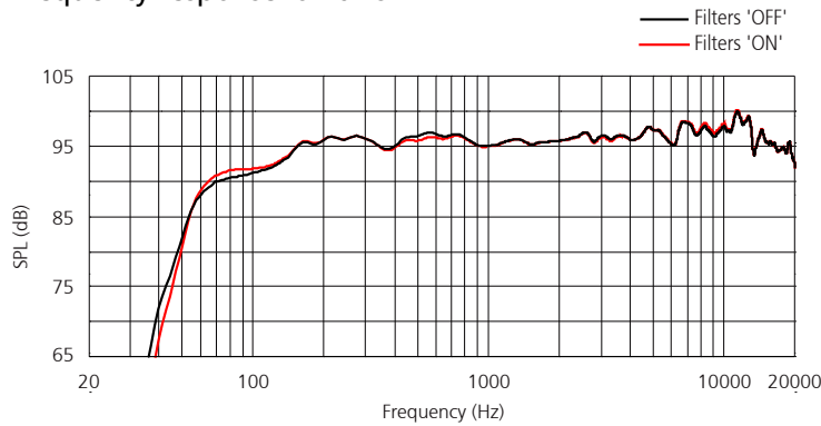
Frequency response 'on axis'
