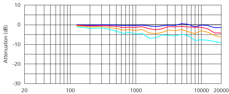
Horizontal frequency response 'off axis'
