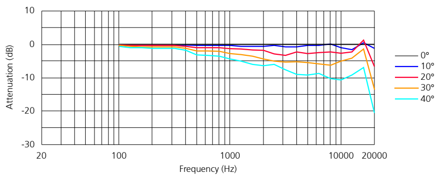
Horizontal frequency response 'off axis'
