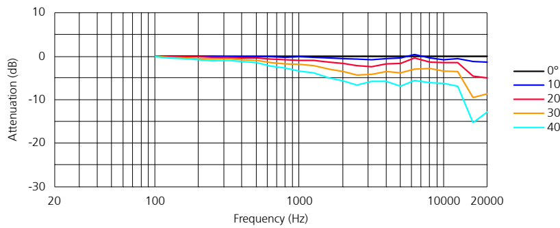
Horizontal frequency response 'off axis'
