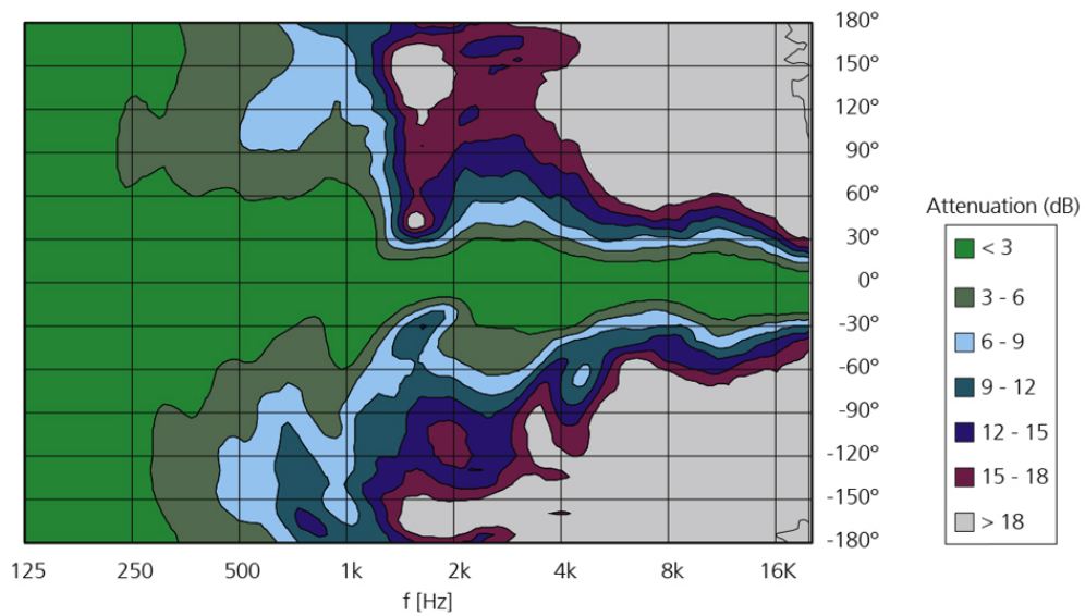
Vertical coverage patter
