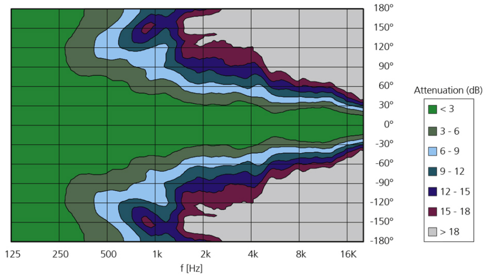
Horizontal coverage patter
