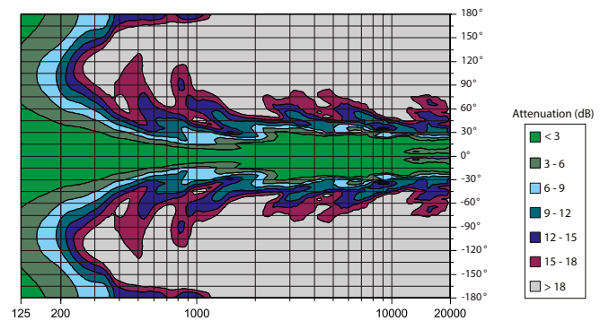
Vertical radiation patten 3 x SEQUENZA 5 W, 15° splayed
