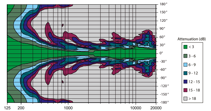
Vertical radiation patten 3 x SEQUENZA 5 W, 9° splayed
