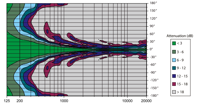
Vertical radiation patten 3 x SEQUENZA 5 W, 3° splayed
