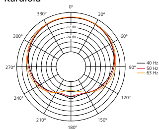
Kardioid
